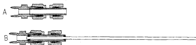
Figure 3. Oven hydrogenator A and injection-port hydrogenator B.
